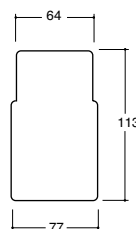
DIFFUSER END CAP FOR LP/LPF
