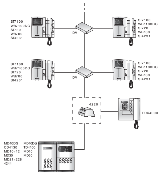
Examples of systems with intercom-telephone-set and PABX's
